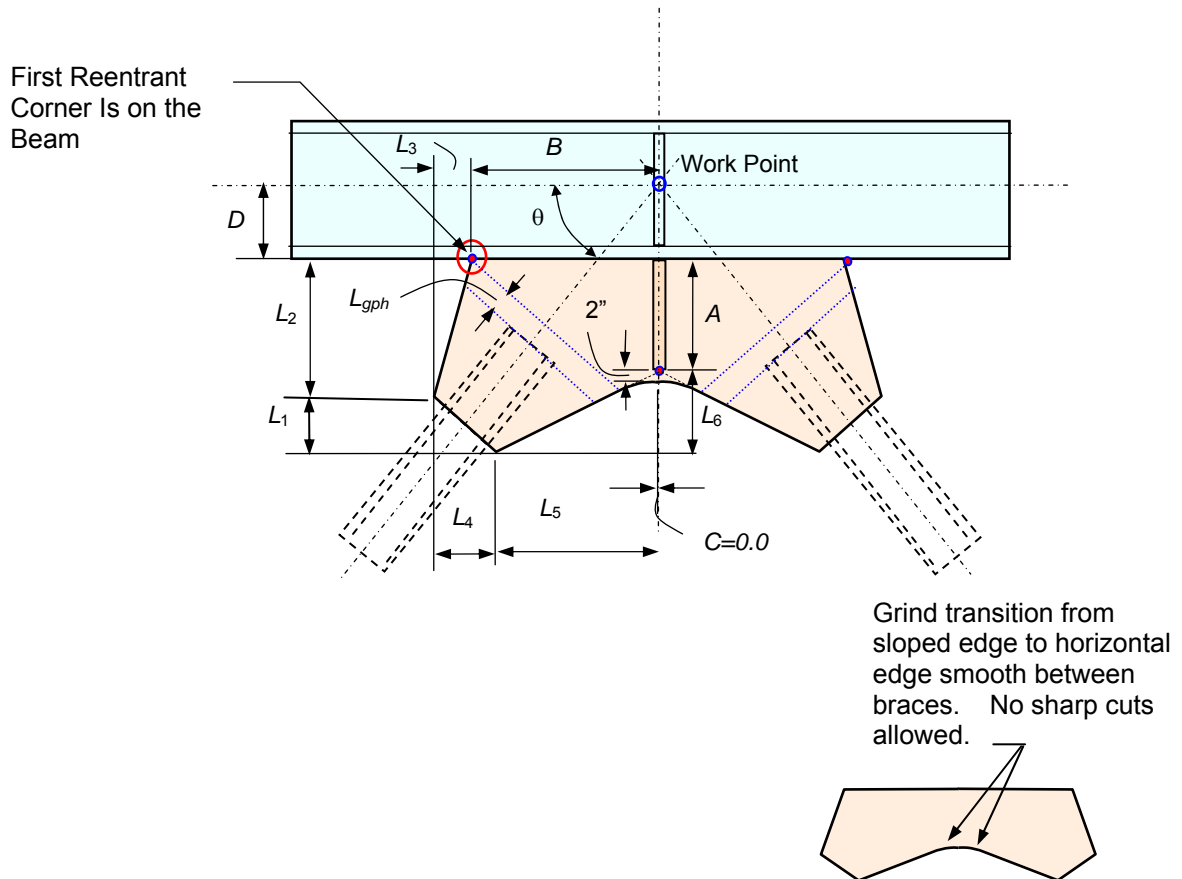
(e) Point of Intersection of the Line of Restraint Is on the Beam
