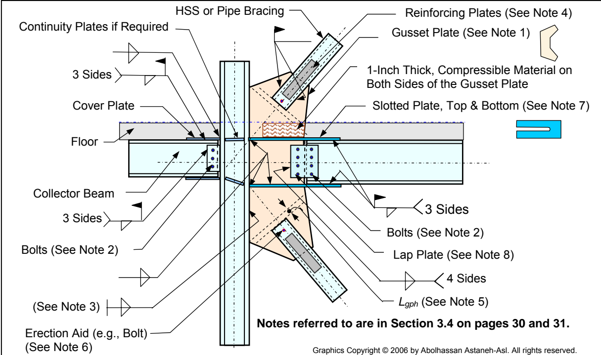
Figure 3.3. Suggested Detail for Gusset Plates of HSS Brace Members (Credit: The above connection was developed by Brian L. Cochran Associates, Inc., Consulting Structural Engineers, Los Angeles, and is presented herein with permission.)
