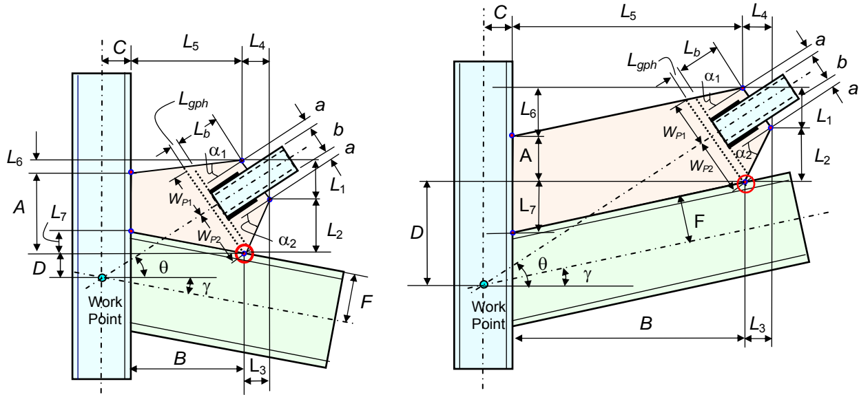
Figure B.6. Sloped Beam with Point of Intersection of the Reentrant Corner on the Beam
