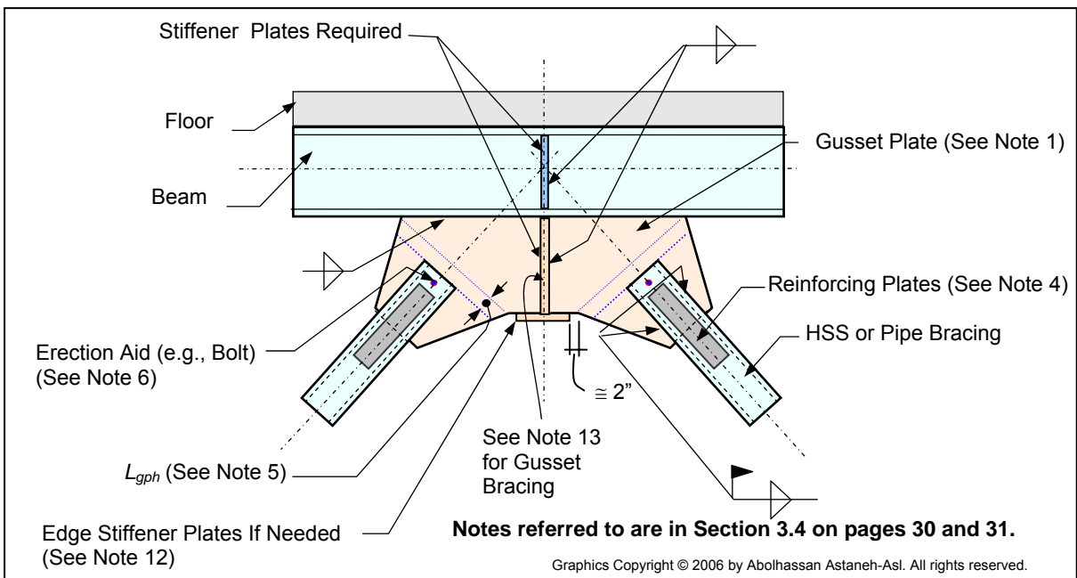
Figure 3.7. Suggested Detail for Gusset Plates of HSS Brace Members
