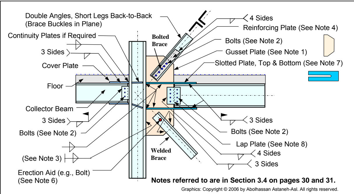
Figure 3.2. Suggested Detail for Gusset Plates of In-Plane Buckling Double Angles (Credit: The above gusset/brace connection for in-plane buckling double-angle braces is taken from Astanteh-Asl, Goel, and Hanson [1982]).
